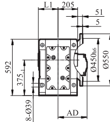
GKA/GKH127
