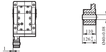
GKH/GKHZ/GKHF127输出轴
