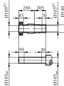
GKH/GKHZ/GKHF127输出轴
