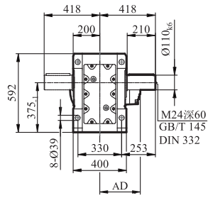
GKA/GKH127
