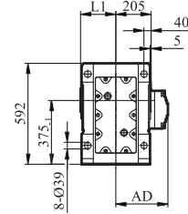
GKA127B GK127B
